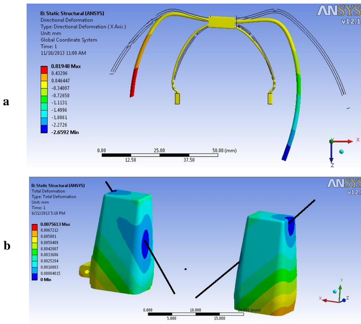
Fig. 3. (a) Outer bow displacement (X5) to show the manner of deformation under loading. (b) Replacing the teeth with two blocks made it easier to show the displacements. The black lines represent the rotation axes (the right band is kept).
