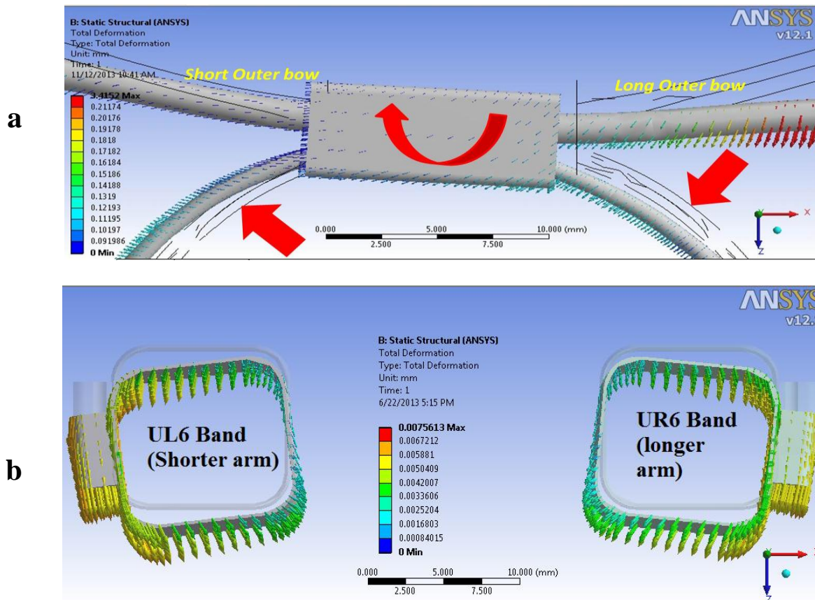
Fig. 7. (a) A closer view of Fig 3a showing the effect of a clockwise moment on the outer bow/inner bow junction. Note the manner of inner bow deformation representing the system yaw. The structure before deformation is shown in thin black lines. (b) An apico-occlusal view of distal movement of the bands (teeth), a rotation caused by the off center force application (the distance between the buccal tube and the tooth long axis), and a clockwise yawing moment; although not easily noticeable (UL6 = upper left first molar; UR6= upper right first
