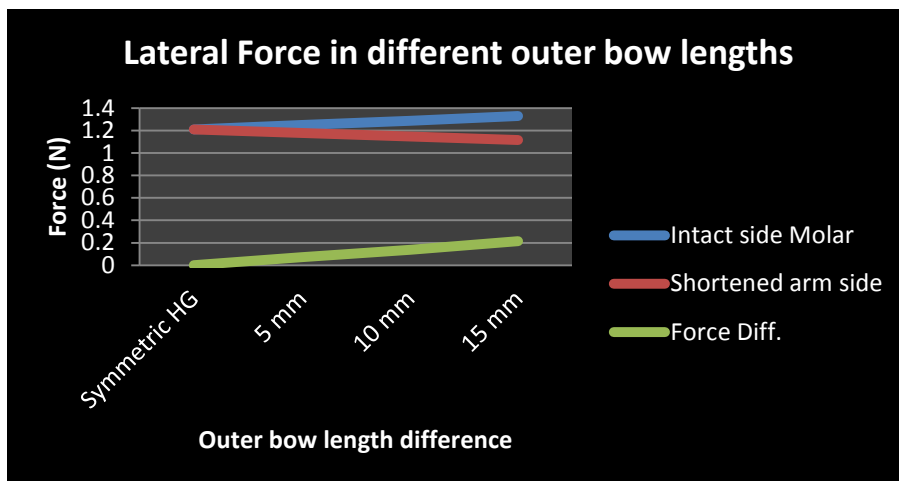
Fig. 4. The influence of asymmetric outer bow on lateral force
