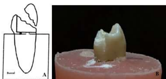
Fig. 2. Schematic (A) and actual (B) reparable mode of failure
