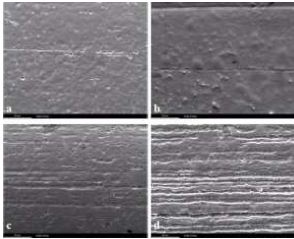
Fig. 5. Surface topography of 0.019x0.025 inch NiTi wires in different subgroups: (a) before immersion, (b) control group, (c) 0.2% NaF group, (d) 0.05% NaF group
