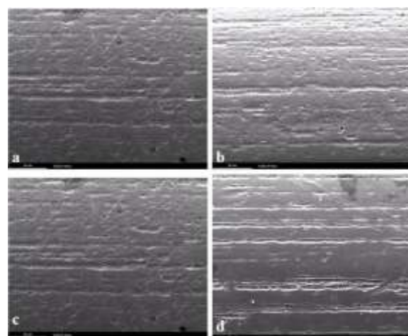
Fig. 3. Surface topography of 0.018-inch NiTi wires in different subgroups: (a) before immersion, (b) control group, (c) 0.2% NaF group, (d) 0.05% NaF group
