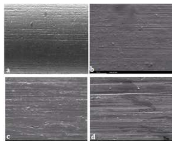
Fig. 4. Surface topography of 0.019x0.025-inch SS wires in different subgroups: (a) before immersion, (b) control group, (c) 0.2% NaF group, (d) 0.05% NaF group
