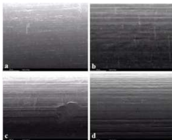
Fig. 2. Surface topography of 0.018-inch SS wires in different subgroups: (a) before immersion, (b) control group, (c) 0.2% NaF group, (d) 0.05% NaF group
