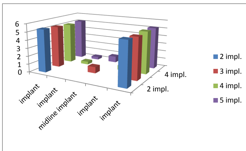
Fig 5. Von Mises stresses on implants.
