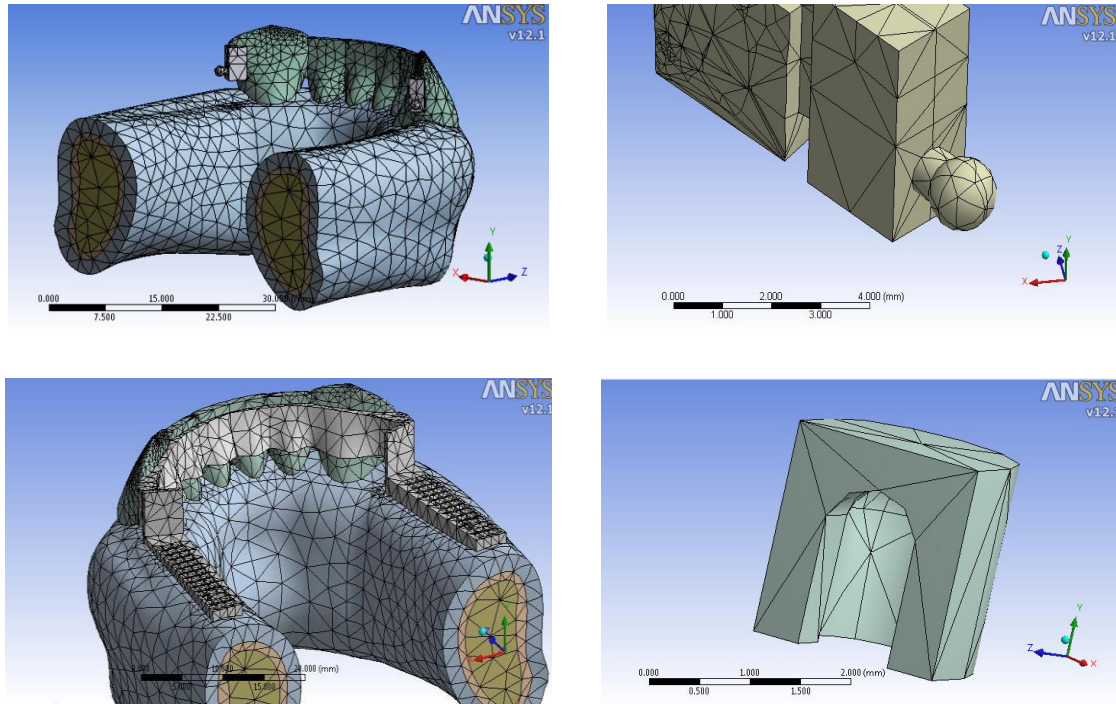
Fig 2. Meshed model. (A) Fixed prosthesis with Patrix part (B) of Dalbo attachment. (C) Fixed and removable part attached by matrix part (D) of Dalbo attachment designed on removable prosthesis
