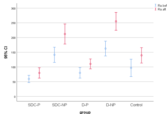
Fig 1. Amount of Ra parameter before and after exposure to demineralization solution. SDC: SWISS denta care; D: Dentaureum; P: Polished; NP: Not-polished.
