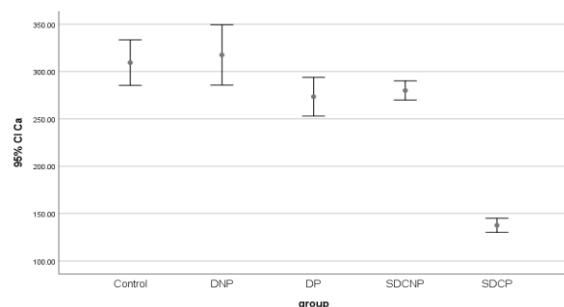
Fig 4. Calcium released (mg/liter) in different groups before and after demineralization. SDC: SWISS denta care; D: Dentaureum; P: Polished; NP: Not-polished.
