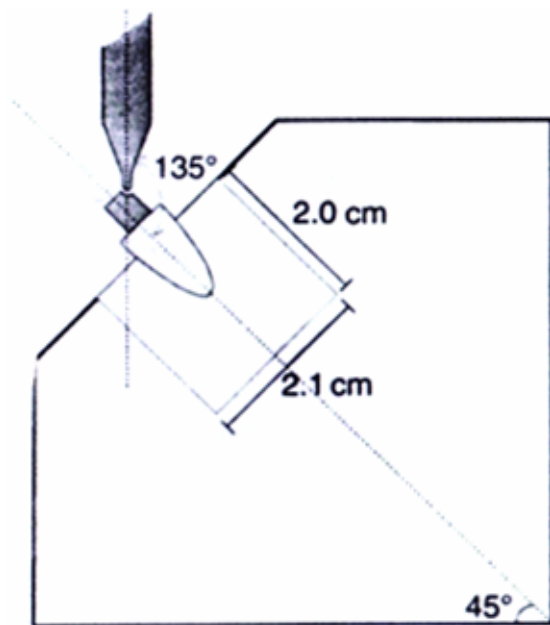
Fig.1: Diagram of the sample holder with the specimen positioned at 45 degrees, took after Mitsui et al [8].
